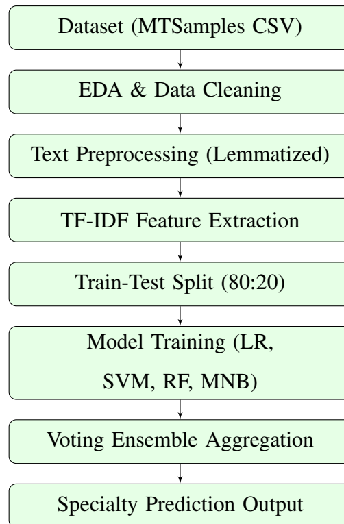
Figure 4: Activity Diagram of the Proposed Machine Learning Algorithm
